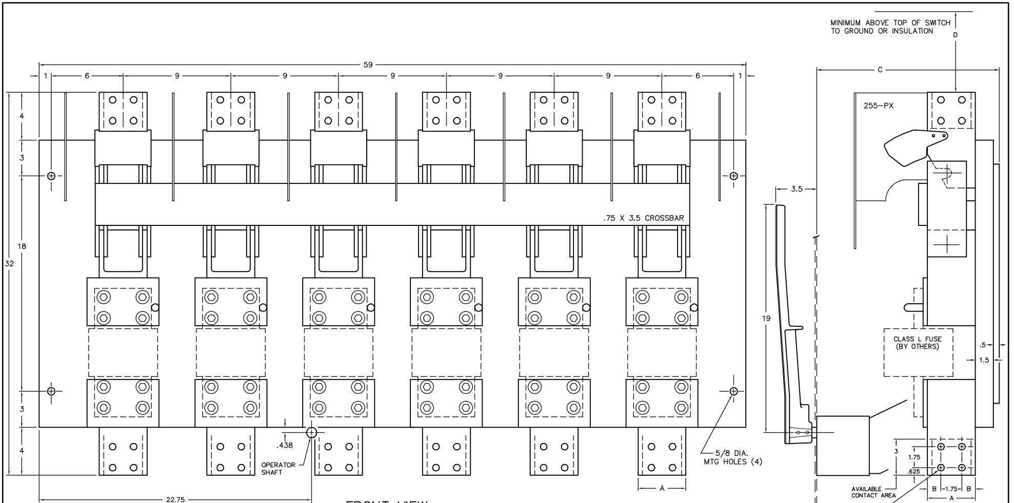
FRONT VIEW
